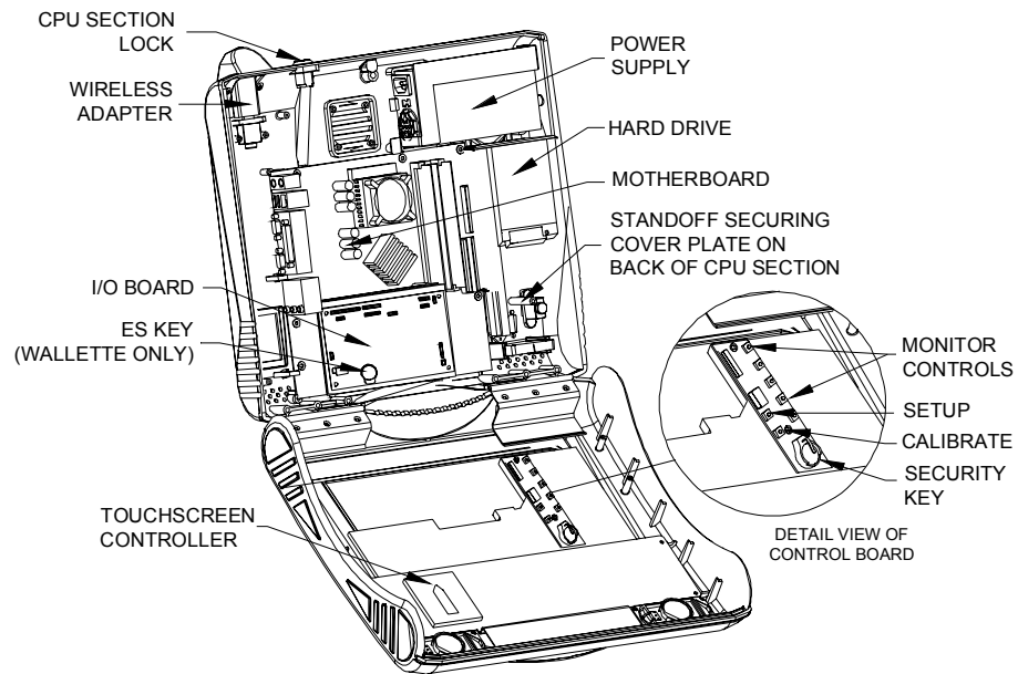
FIGURE A- WALLETTE / ENTERTAINER WITH CPU SECTION OPEN
