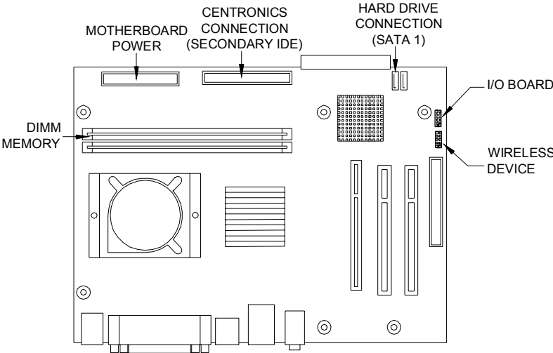
TOP VIEW OF MOTHERBOARD
