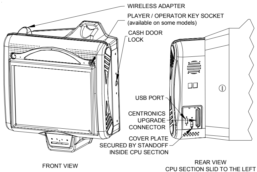
FIGURE B - FRONT AND REAR VIEWS OF WALLETTE / ENTERTAINER
