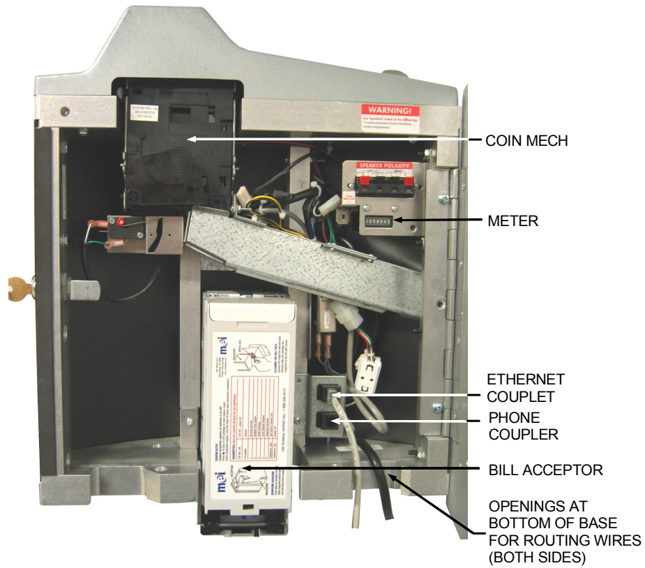
FIGURE E - BACK OF WALLETTTE / ENTERTAINER- CASH DOOR OPEN
