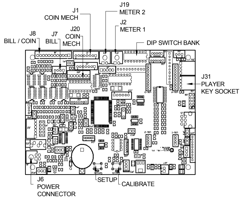
FIGURE 34 - I/O BOARD DRAWING
