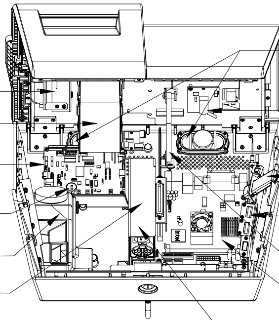
REAR VIEW OF AN OPEN MEGATOUCH ION RX
