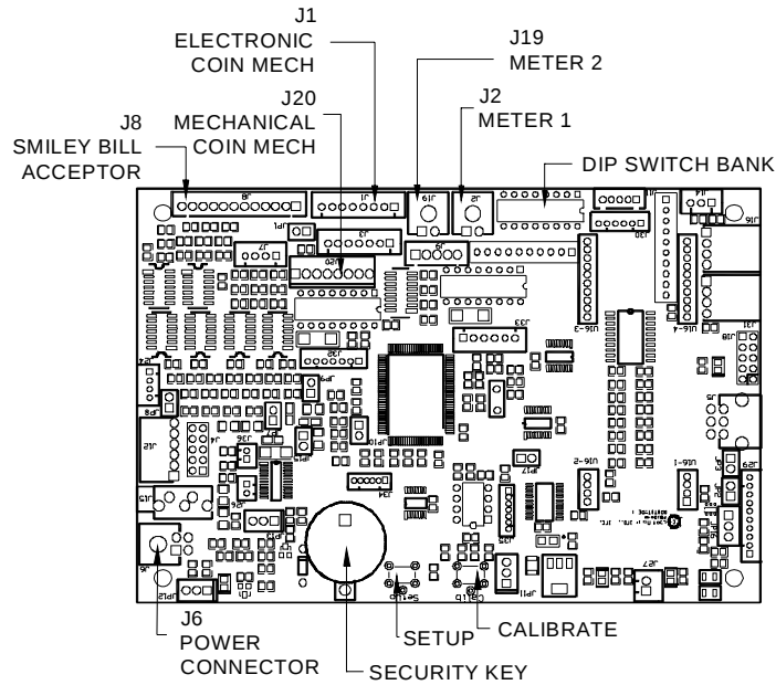
FIGURE 34 - I/O BOARD DRAWING
