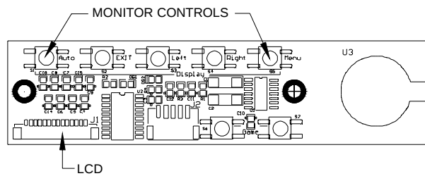
FIGURE 35 - ON-SCREEN DISPLAY BOARD DRAWING
