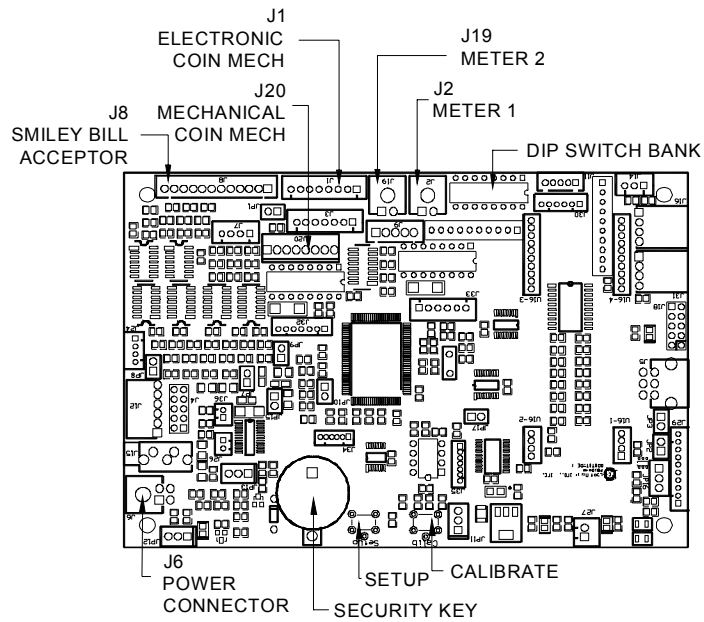
FIGURE 38 - I/O BOARD DRAWING
