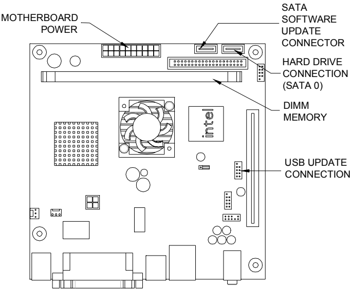
TOP VIEW OF MOTHERBOARD
