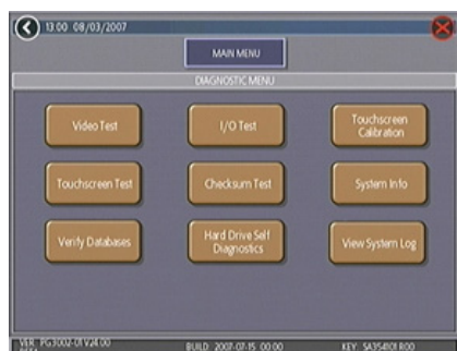
FIGURE 15 - DIAGNOSTICS MENU
