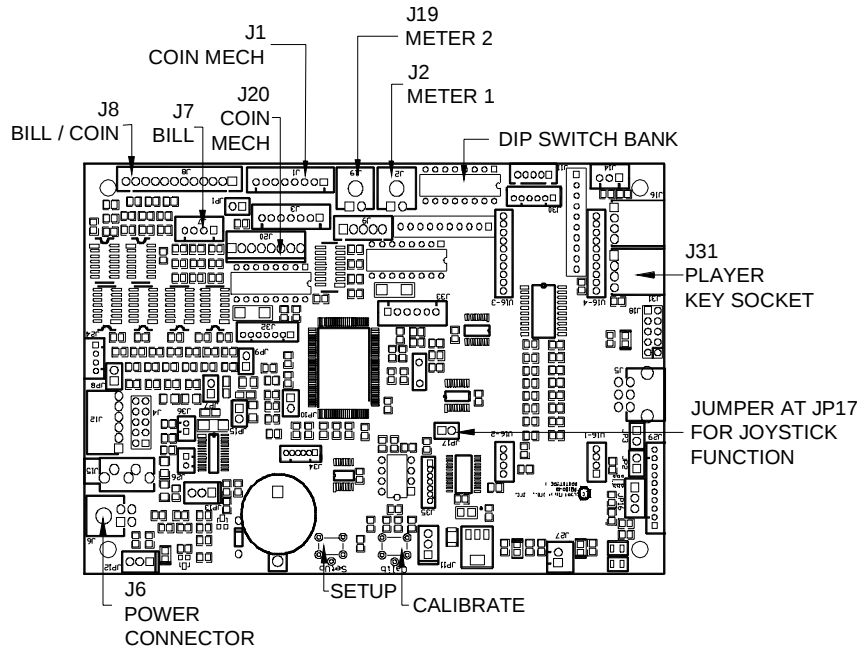
FIGURE 38 - I/O BOARD DRAWING
