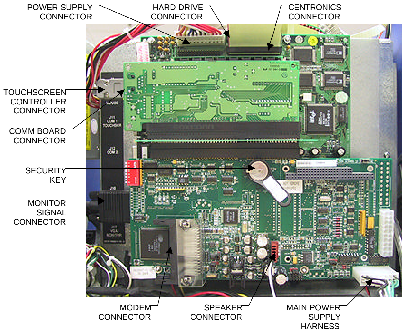
FIGURE 3 - TELCO MOTHERBOARD
