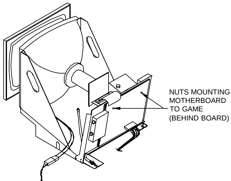
FIGURE 1 - BLUE MAXX/MAXX CLASSIC - MOTHERBOARD REMOVAL
