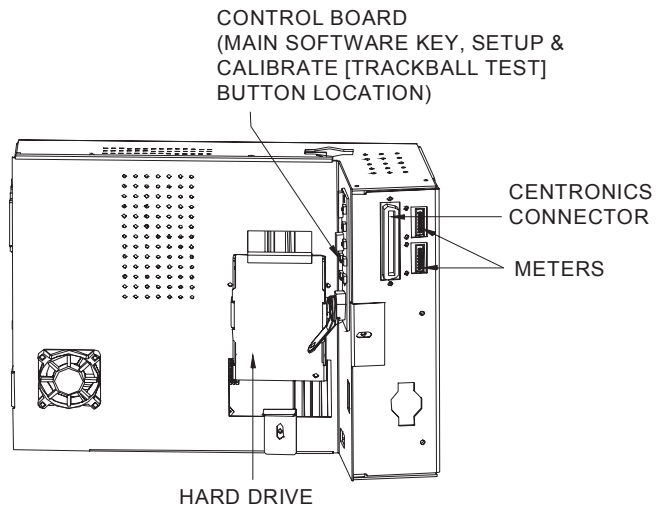
DETAIL VIEW OF ELECTRONICS BOX WITH COVER ON
