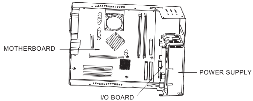
DETAIL VIEW OF ELECTRONICS BOX WITH COVER REMOVED
