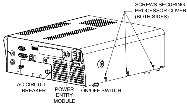
FIGURE 17 - FORCE VIBE WITH COVER
