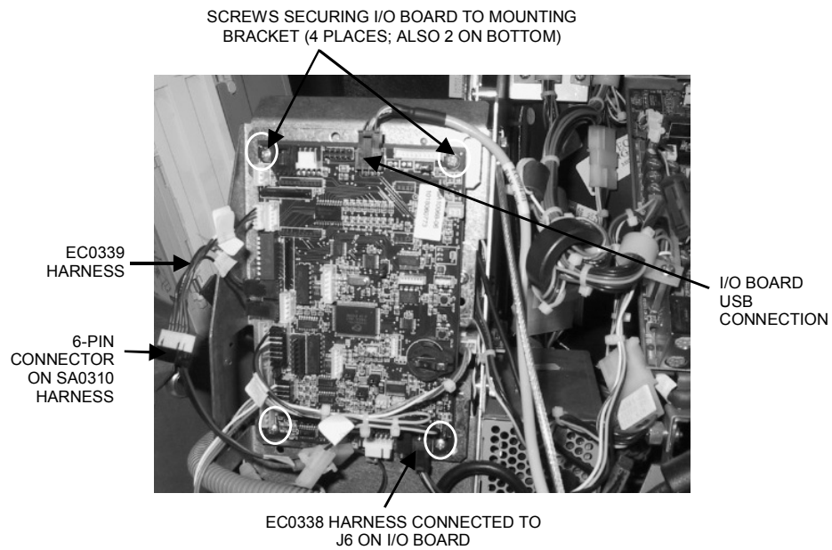
FIGURE 8 - NEW I/O BOARD IN RADION GAME
