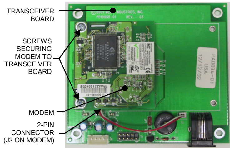
FIGURE 10 - MODEM ASSEMBLY - MODEM AND TRANSCIVER BOARD
